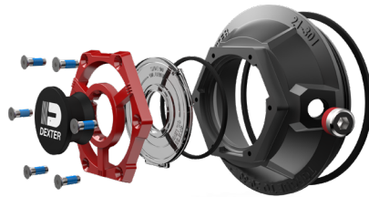
THREADED CAP
